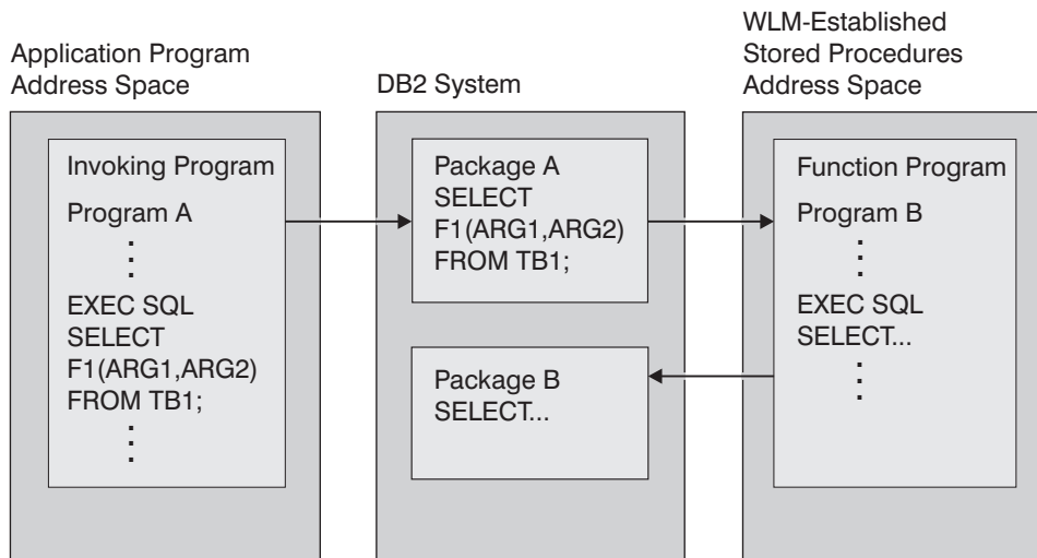
Figure 26. The user-defined function environment
