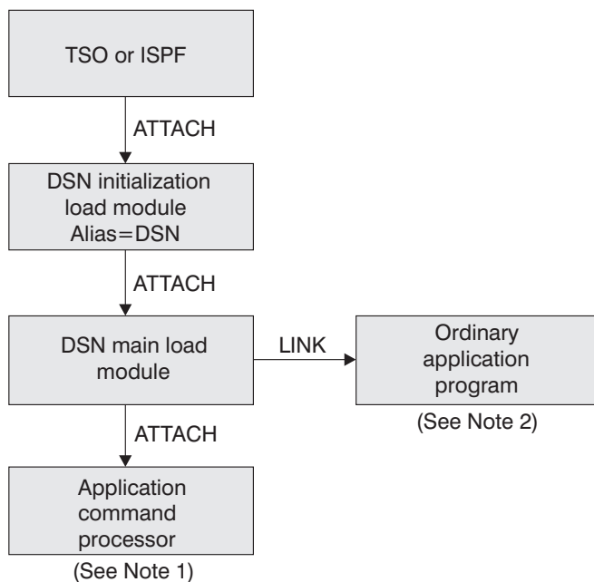
Figure 74. DSN task structure
