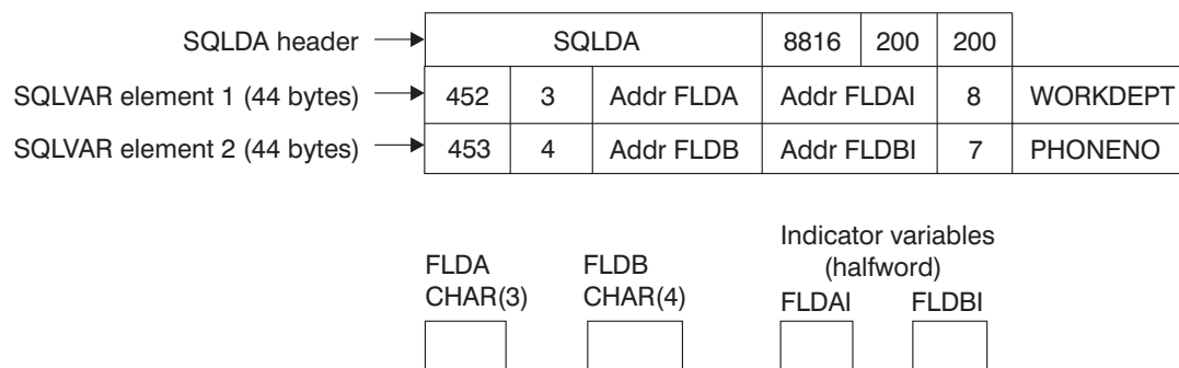
Figure 15. SQL descriptor area after analyzing descriptions and acquiring storage
