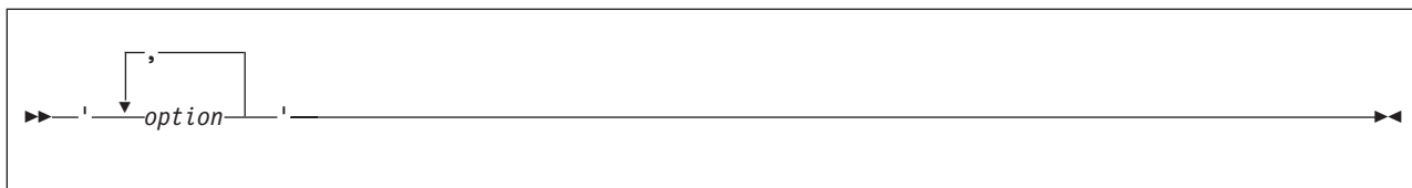
Figure 32. CALL DSNTPSMP bind-options, compiler-options, precompiler-options, prelink-options, link-options
