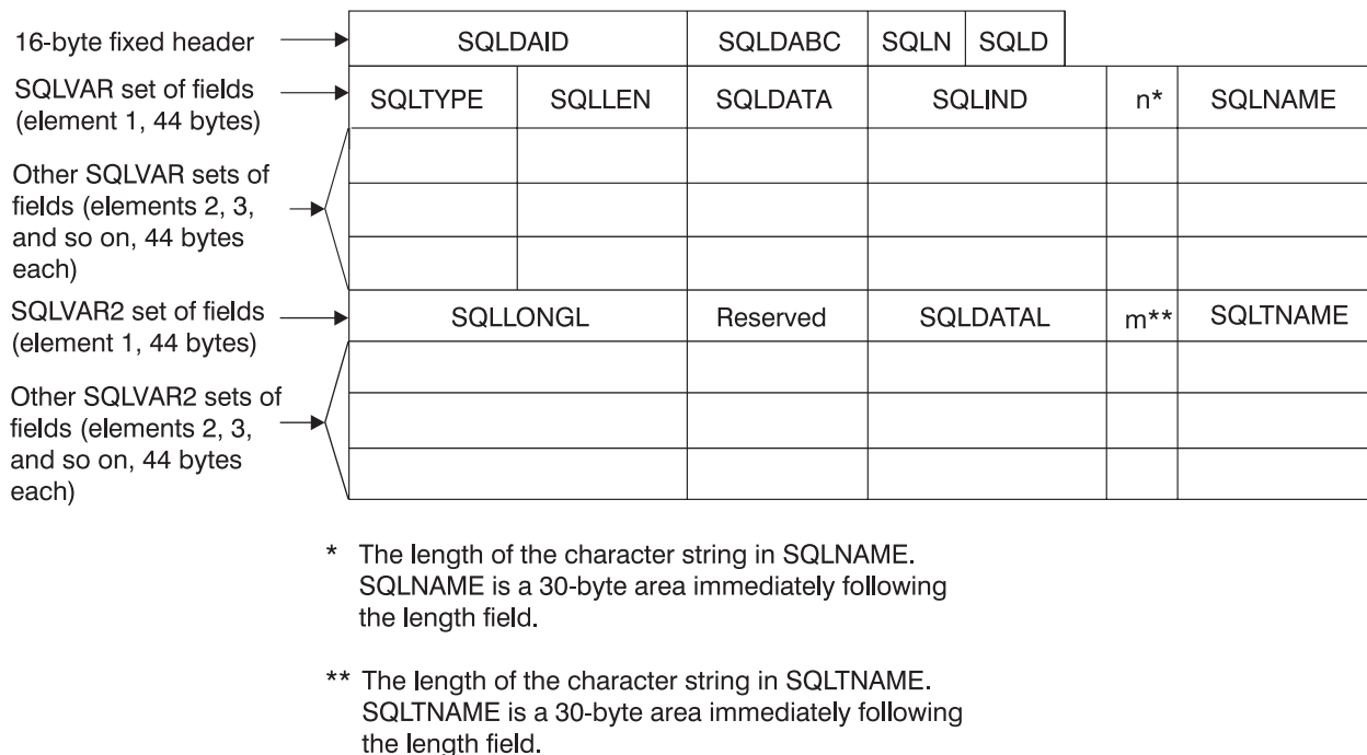
Figure 13. The full-size SQLDA structure
