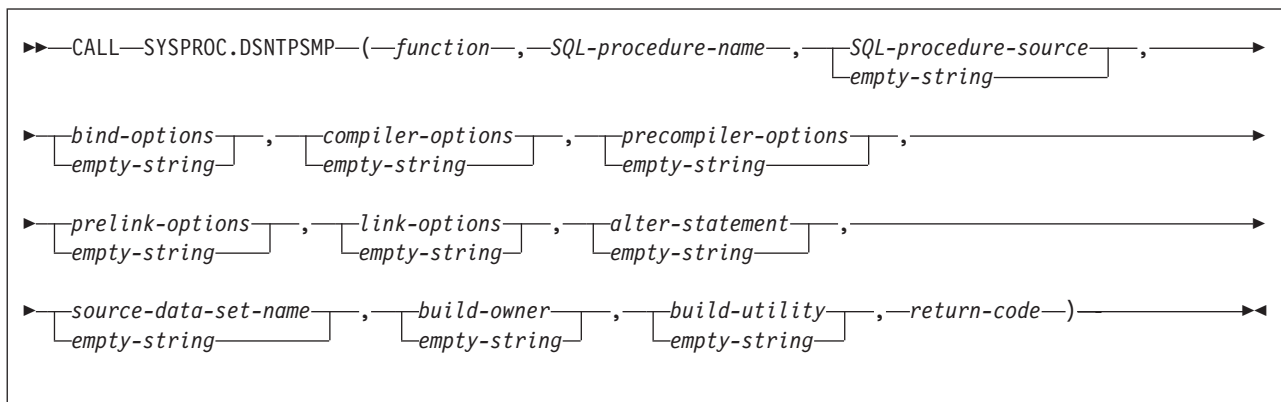
Figure 31. DSNTPSMP syntax
