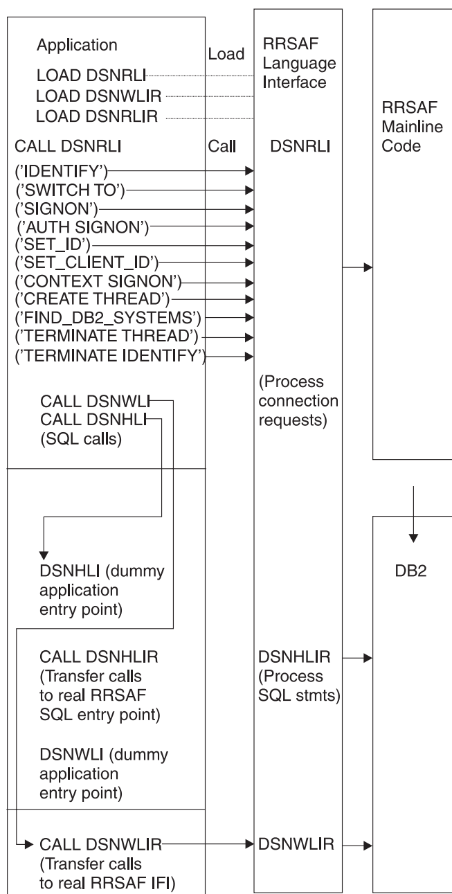
Figure 3. Sample RRSAP configuration
